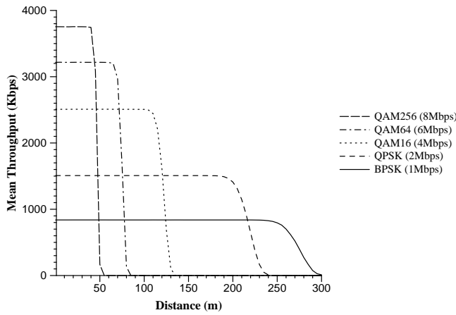
Figure 2: Comparison of throughput versus distance for several modulation schemes. Data was obtained by the simulation of two nodes at fixed positions, with one sending a continuous stream of UDP packets to the other. The propagation model was the log-distance path loss model, with a path loss exponent typical of an urban environment. Transmit power was constant.
