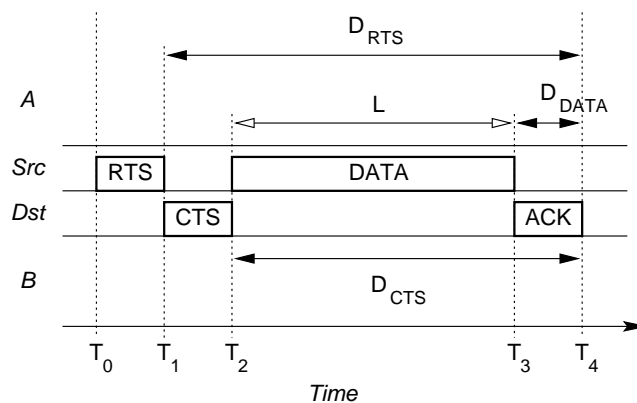
Figure 4: Timeline showing the RTS/CTS protocol in the IEEE 802.11 Distributed Coordination Function (DCF) for transmitting a data packet. Here, A and B are nodes that are in range of the transmitter and receiver, respectively. D_{RTS} , D_{CTS} , and D_{DATA} are the lengths of the reservations given in the RTS, CTS and DATA packets, and L is the duration of the data packet transmission.
